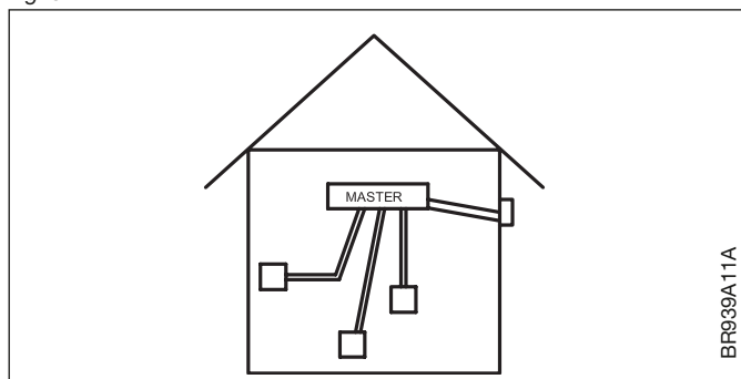
Sensors and outdoor compensation module connected in star formation
